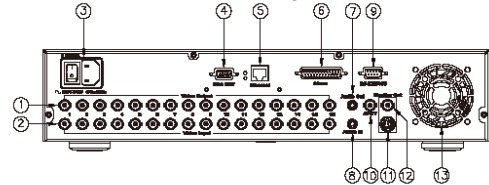
Back Panel Layout
